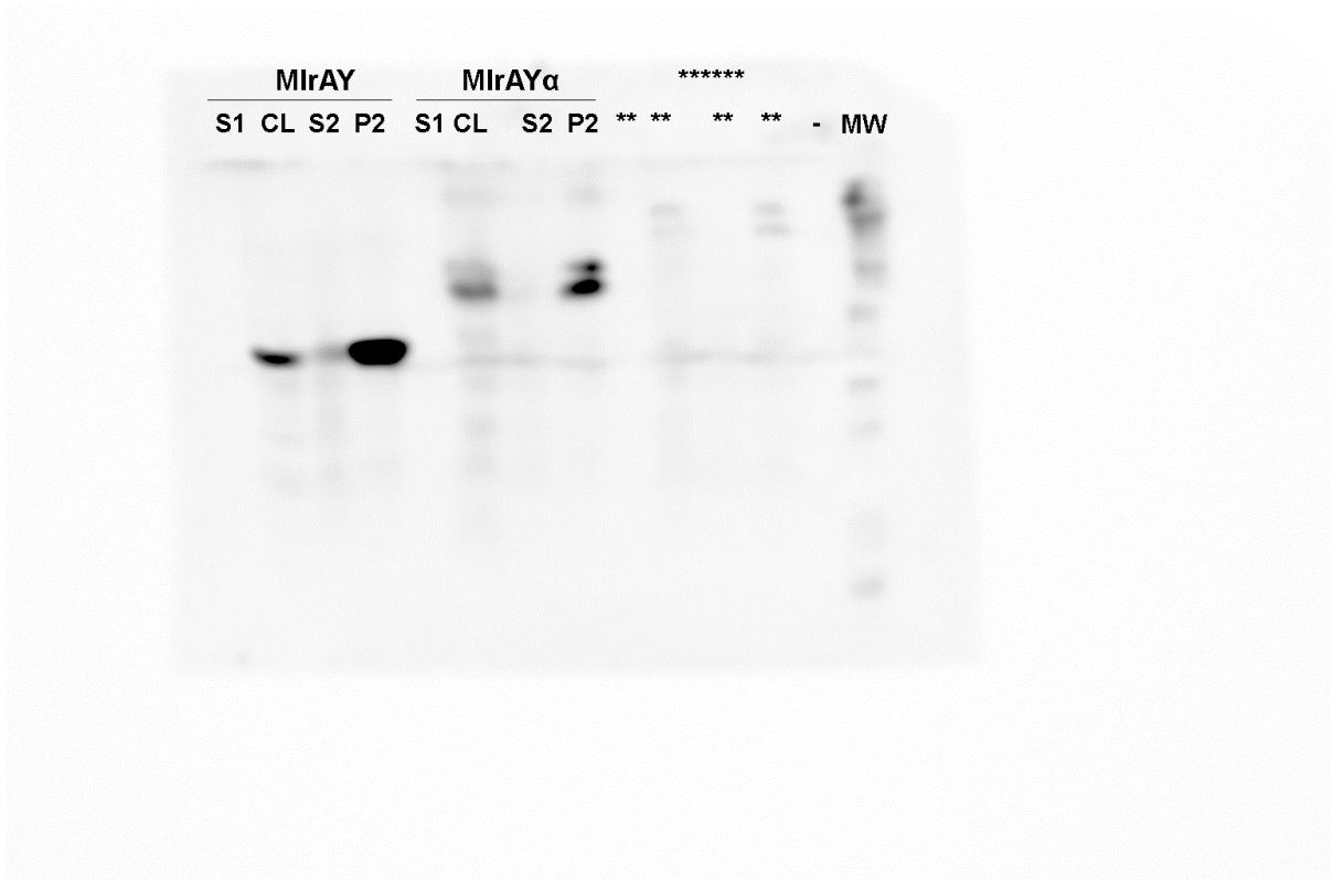
Expression ECL
